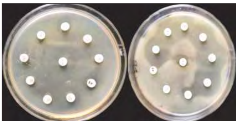
Fig.3. Antibiotic Sensitivity pattern of Clostridium perfringens Mueller Hinton agar (MHA) plates
