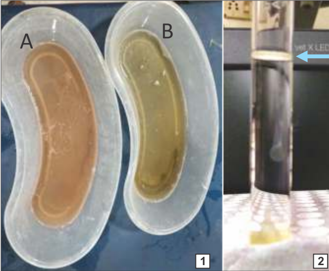
Fig. 1a. Watery, slimy and red tinged peritoneal fluid and 1B. Transparent, pale yellowish pleural fluid Fig. 2. Rivalta's test–Retained jelly-fish-like drop attached to the surface and floats down to the bottom of the tube
